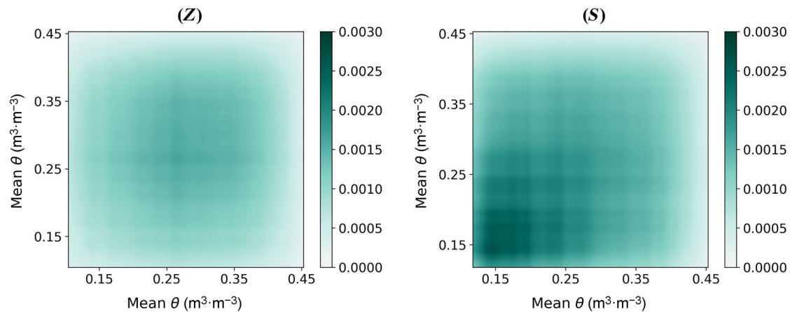
FIGURE 6 SM: Covariance matrices in function of mean soil moisture contents based on virtual observed soil moisture variability for the depth-dependent (Z) and structure-dependent (S) root distribution, after applying a Gaussian filter with a standard deviation of 10 soil moisture steps.
